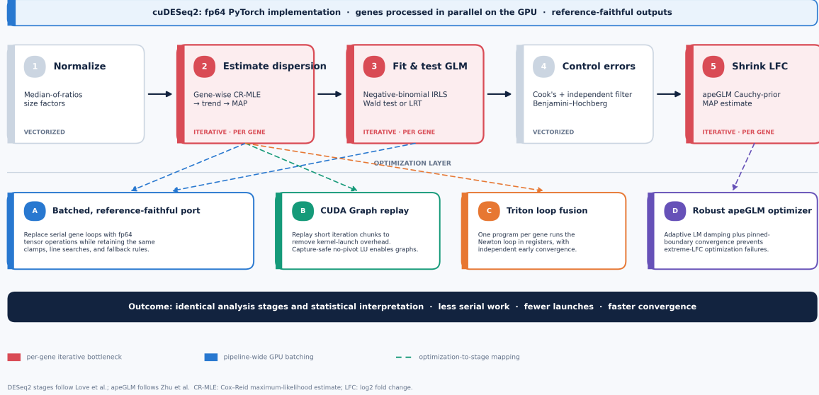
Figure 1 | DESeq2 workflow and cuDESeq2 optimization strategy
