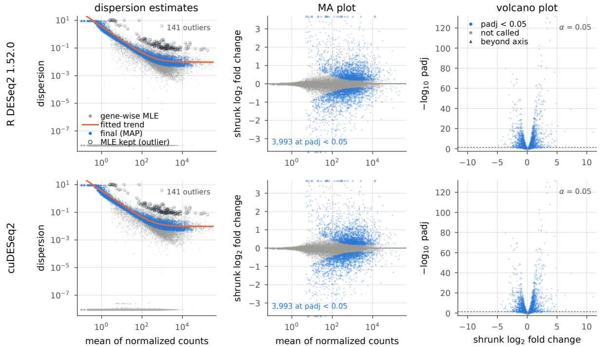
Figure 3: The three standard DESeq2 diagnostics on airway ( \sim \text{cell} + \text{dex} , n=8 , P=5 ), drawn from R DESeq2 1.52.0 (top) and cuDESeq2 (bottom) by the same plotting code. Left , the plotDispEsts view: gene-wise MLE (grey), fitted trend (orange), final estimate (blue), and circled genes whose MLE exceeds the trend by more than two residual SDs and is therefore kept unshrunk. Center , MA plot of the apeGLM-shrunk LFC, with out-of-range genes on the boundary as in plotMA . Right , volcano plot. Axis limits are computed from R's output and reused for cuDESeq2.
