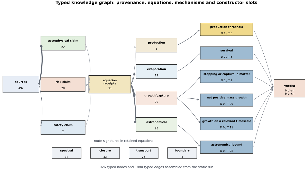
Figure 4: Typed knowledge graph assembled from the static run. It contains 926 typed nodes and 1,880 typed edges. The left side is provenance; the middle is the retained equation layer; the right side is the constructor layer that decides whether the danger branch closes.
