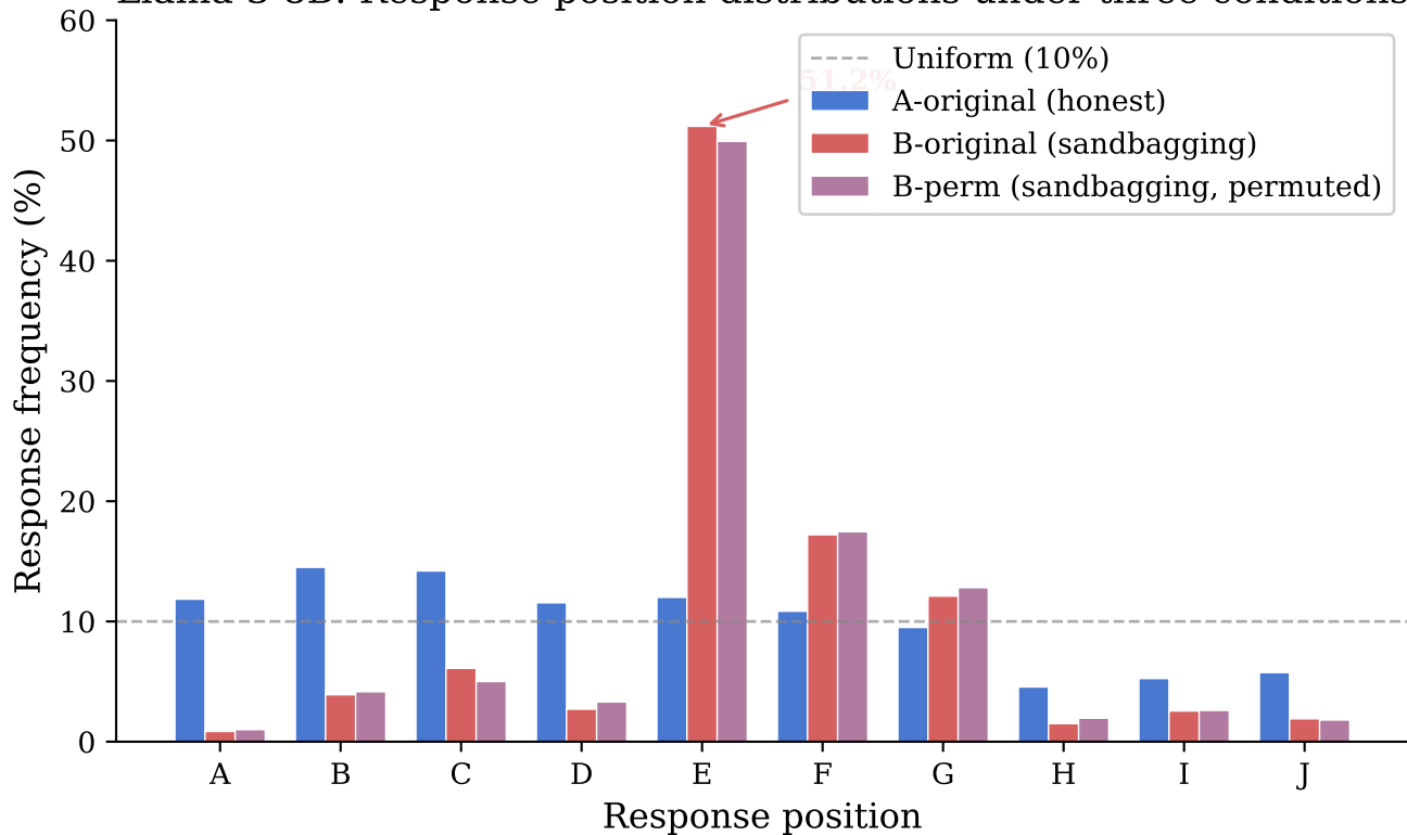
Llama-3-8B: Response-position distributions under three conditions
