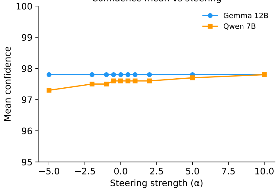
Confidence mean vs steering
