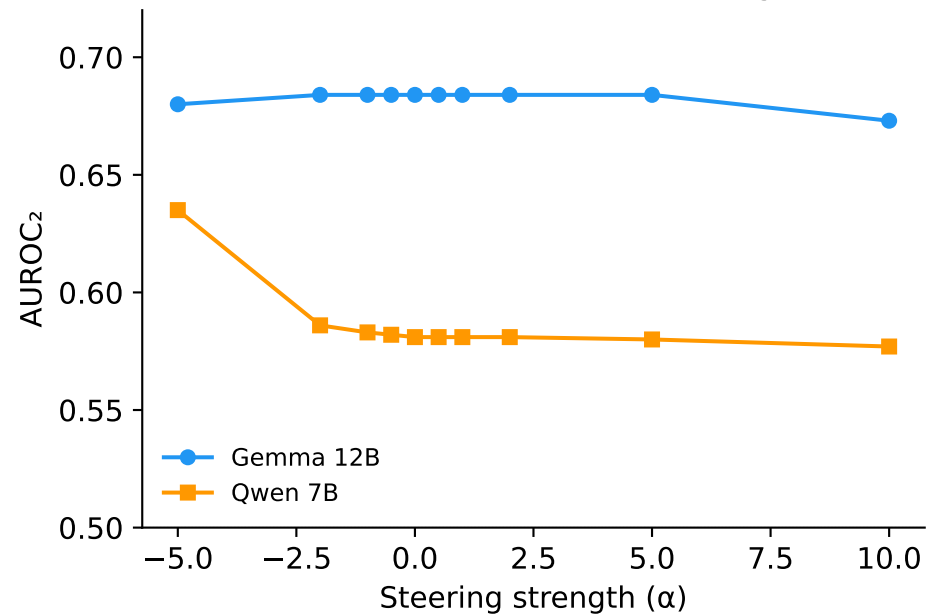
Verbal discrimination vs steering
