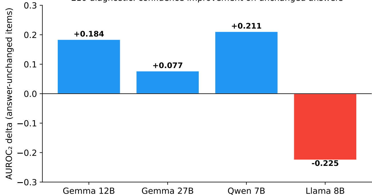
E10 diagnostic: confidence improvement on unchanged answers
