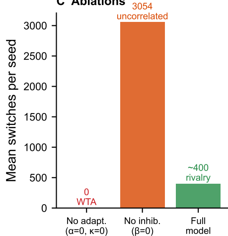
C Ablations
