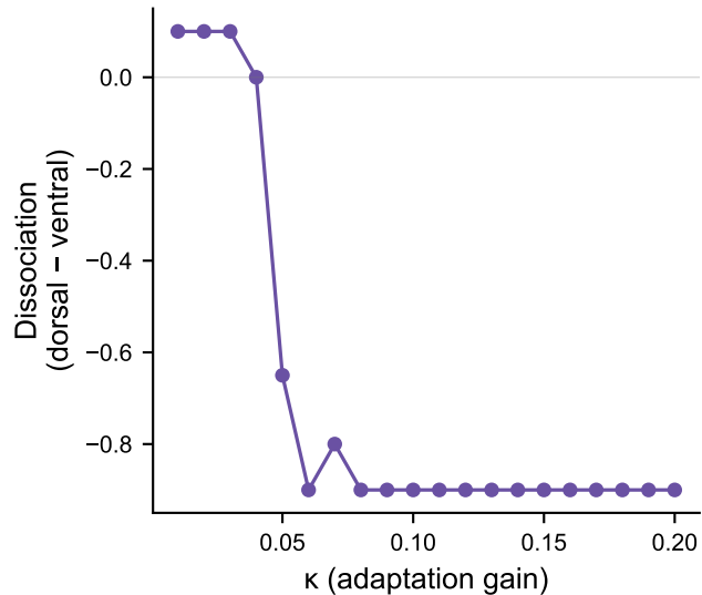
C Dissociation vs \kappa
