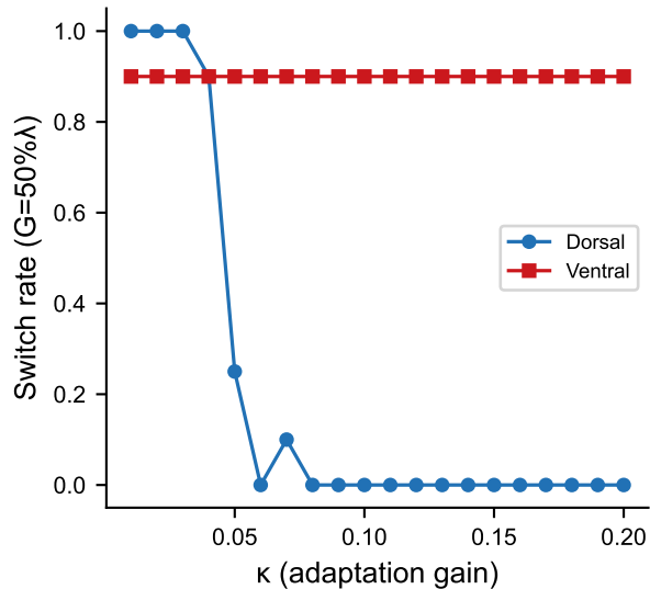
B Controllability vs \kappa
