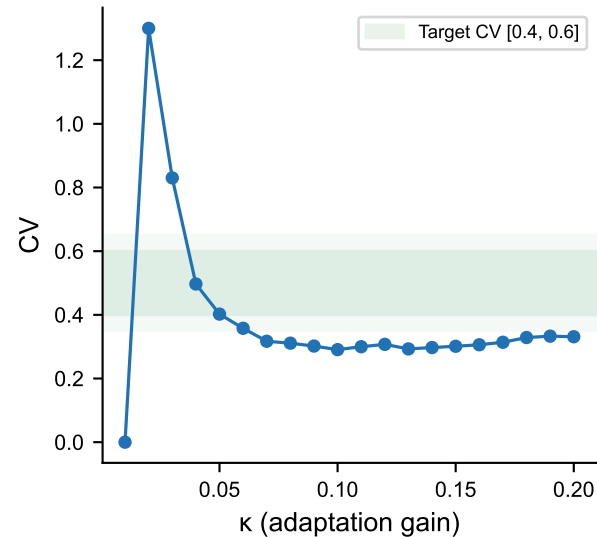
A CV vs \kappa
