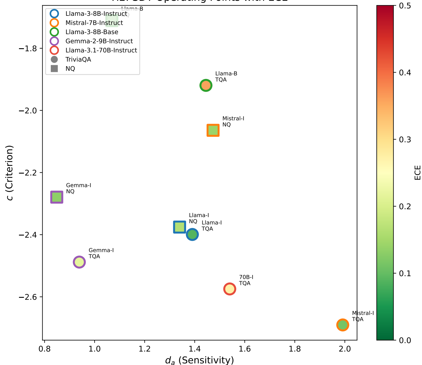
H2: SDT Operating Points with ECE
