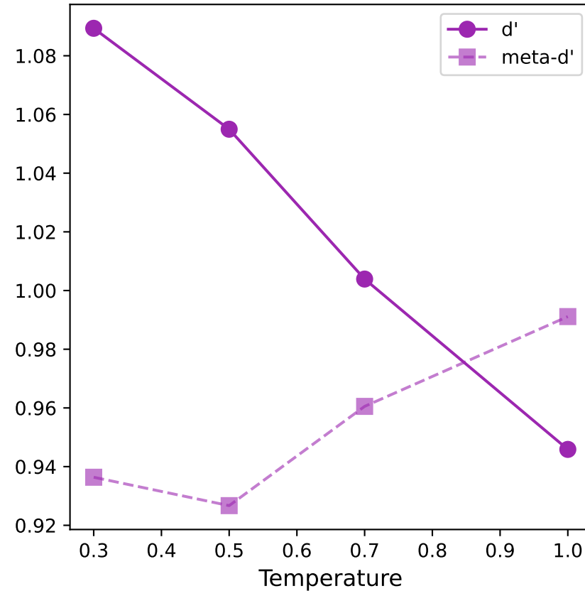
Gemma-2-Instruct \rho(\text{meta-d}', T) = +0.80 , \rho(d', T) = -1.00
