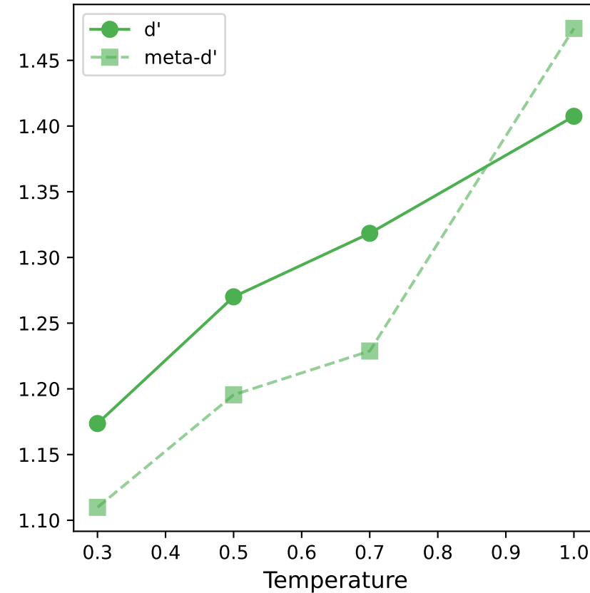
Llama-3-Base \rho(\text{meta-d}', T) = +1.00 , \rho(d', T) = +1.00
