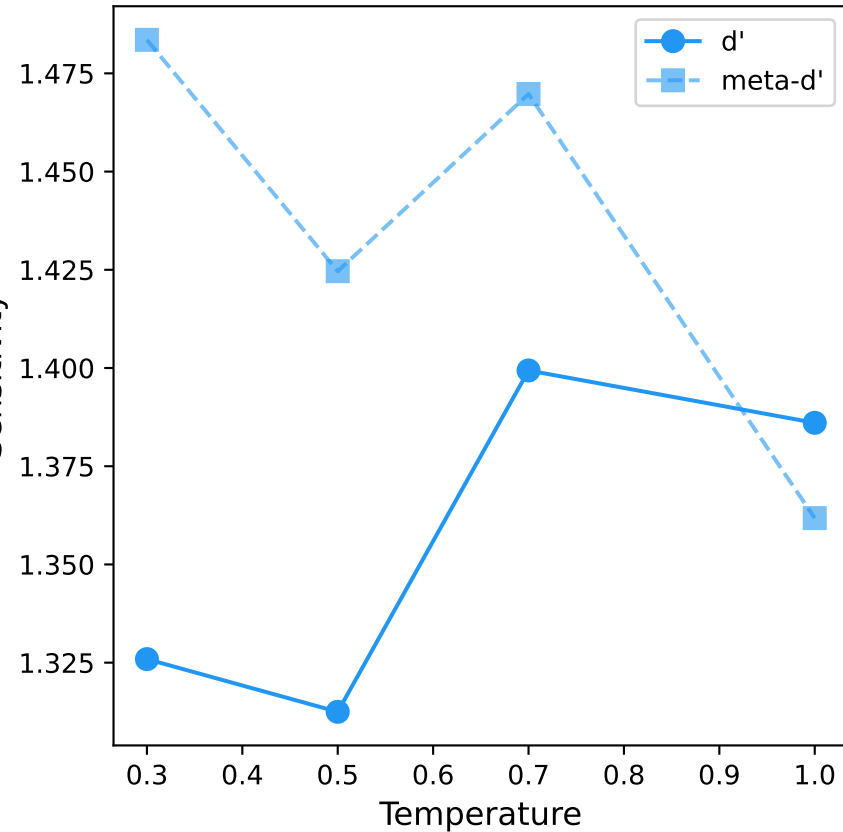
Llama-3-Instruct \rho(\text{meta-d}', T) = -0.80 , \rho(d', T) = +0.60
