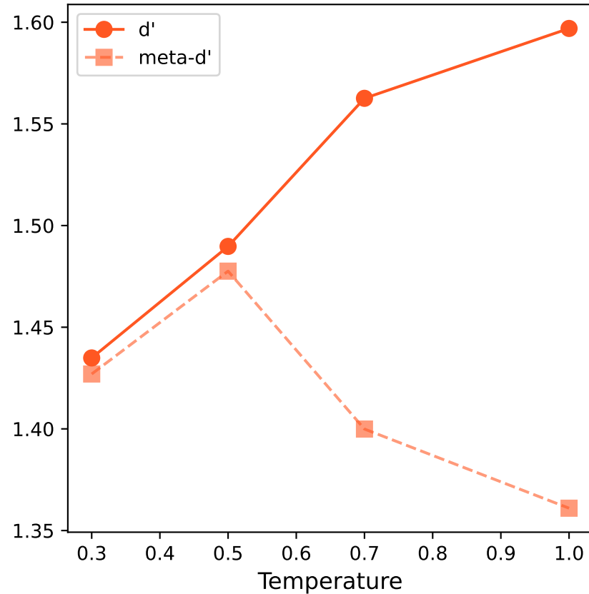
Mistral-Instruct \rho(\text{meta-d}', T) = -0.80 , \rho(d', T) = +1.00
