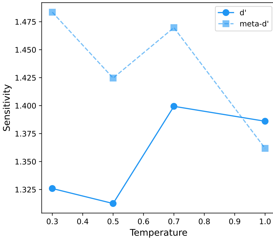
Llama-3-Instruct \rho(\text{meta-d}', T) = -0.80 , \rho(d', T) = +0.60
