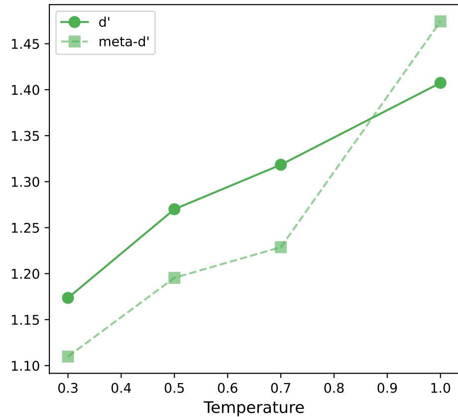
Llama-3-Base \rho(\text{meta-d}', T) = +1.00 , \rho(d', T) = +1.00
