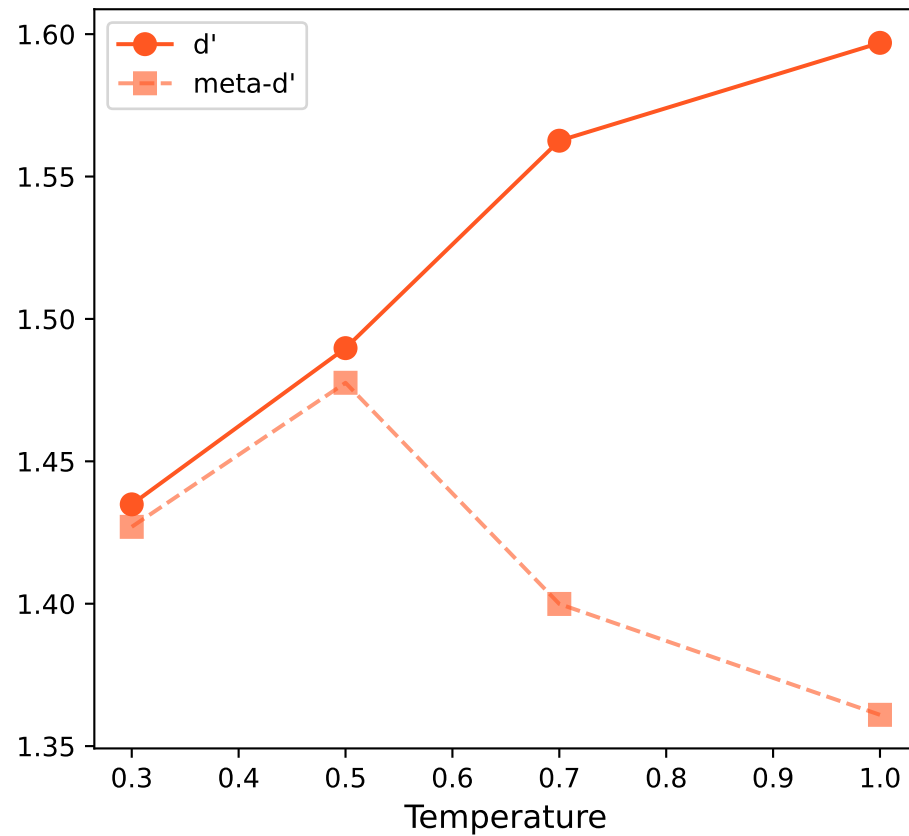
Mistral-Instruct \rho(\text{meta-d}', T) = -0.80 , \rho(d', T) = +1.00
