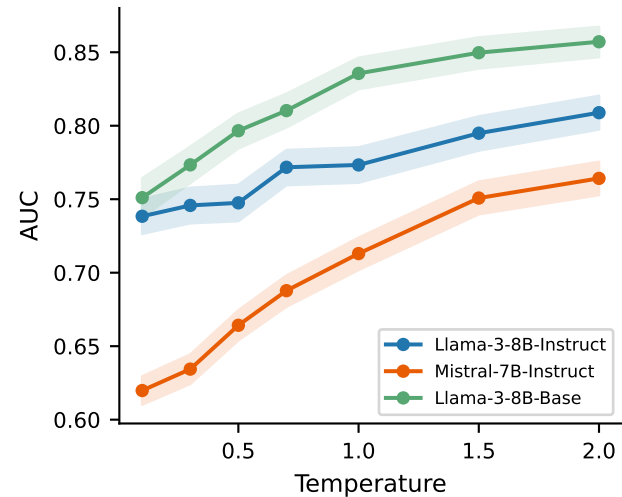
AUC vs Temperature (TQA)
