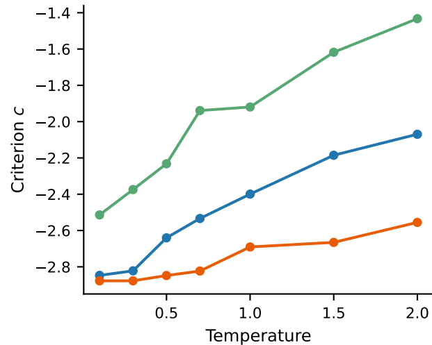
Criterion vs Temperature (TQA)
