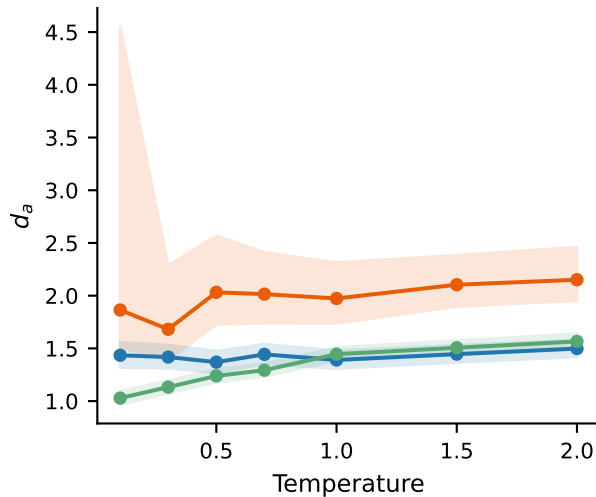
d_a vs Temperature (TQA)
