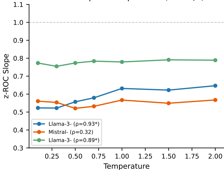
z-ROC Slope \times Temperature (TriviaQA)
