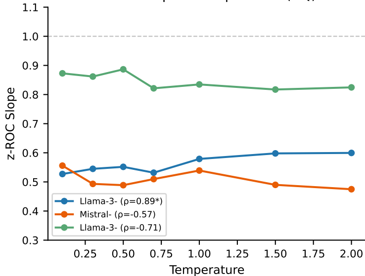
z-ROC Slope \times Temperature (NQ)
