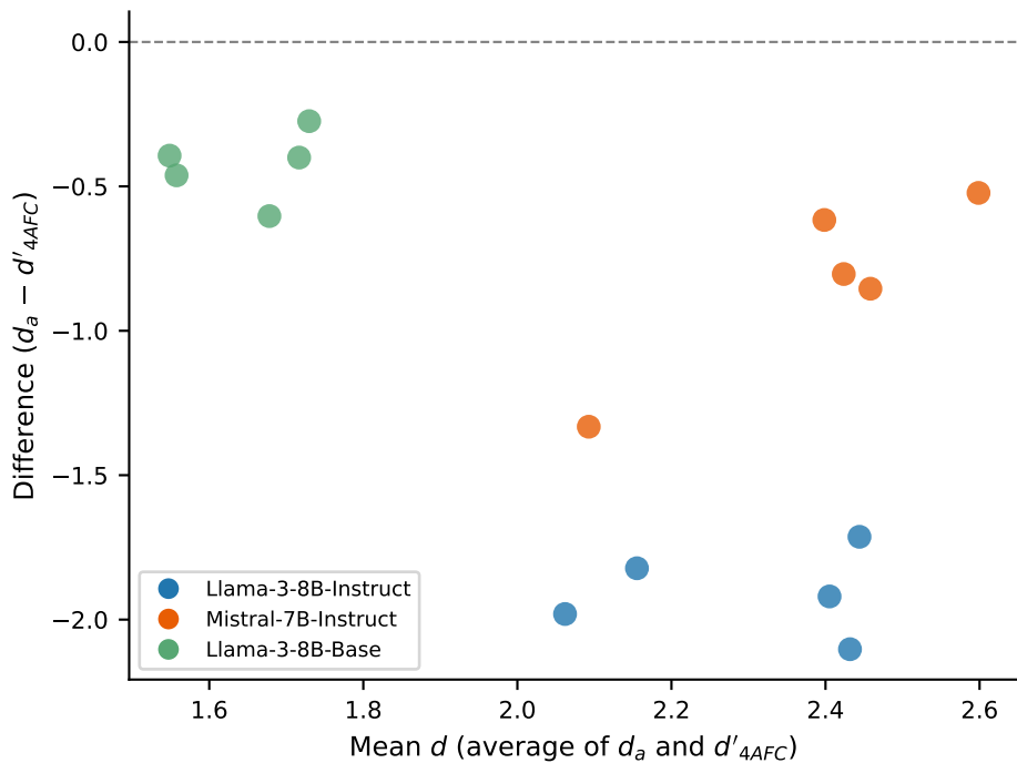
H3: Bland-Altman — Paradigm A vs B
