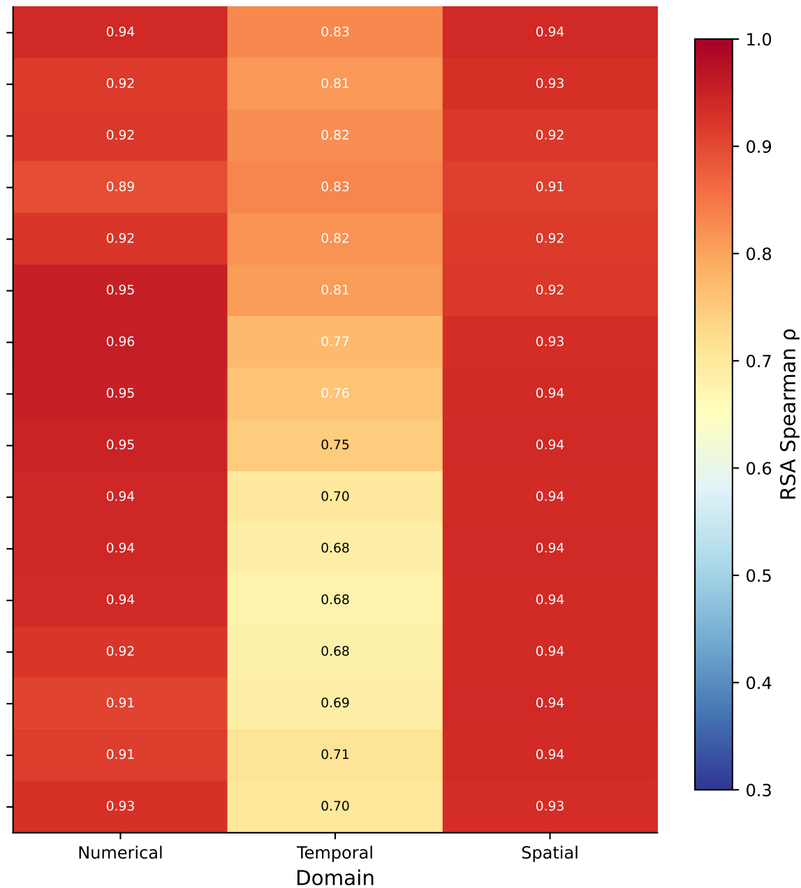
Mistral-7B-Instruct-v0.3
