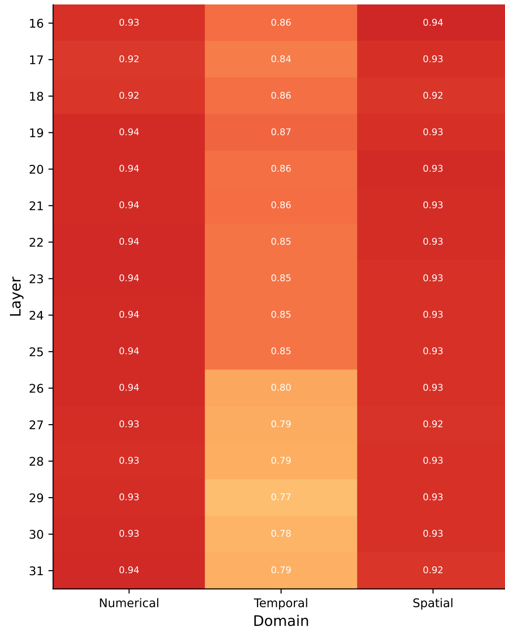
Llama-3-8B-Instruct
