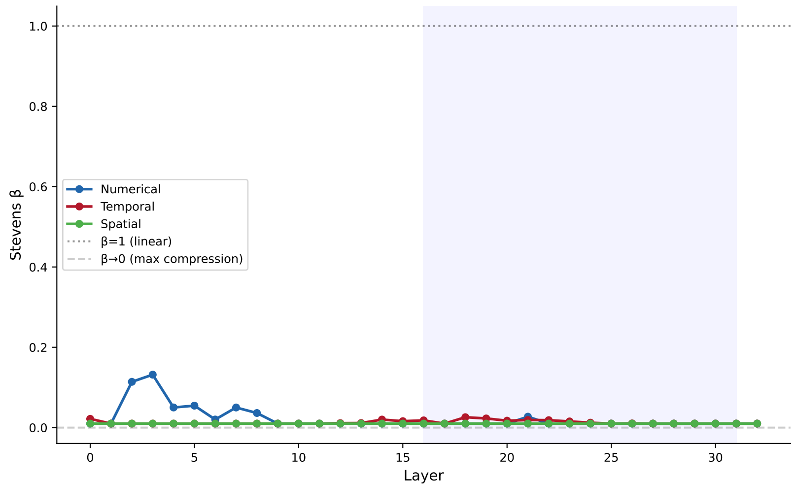
F8: Stevens \beta Across Layers — Mistral-7B-Instruct-v0.3
