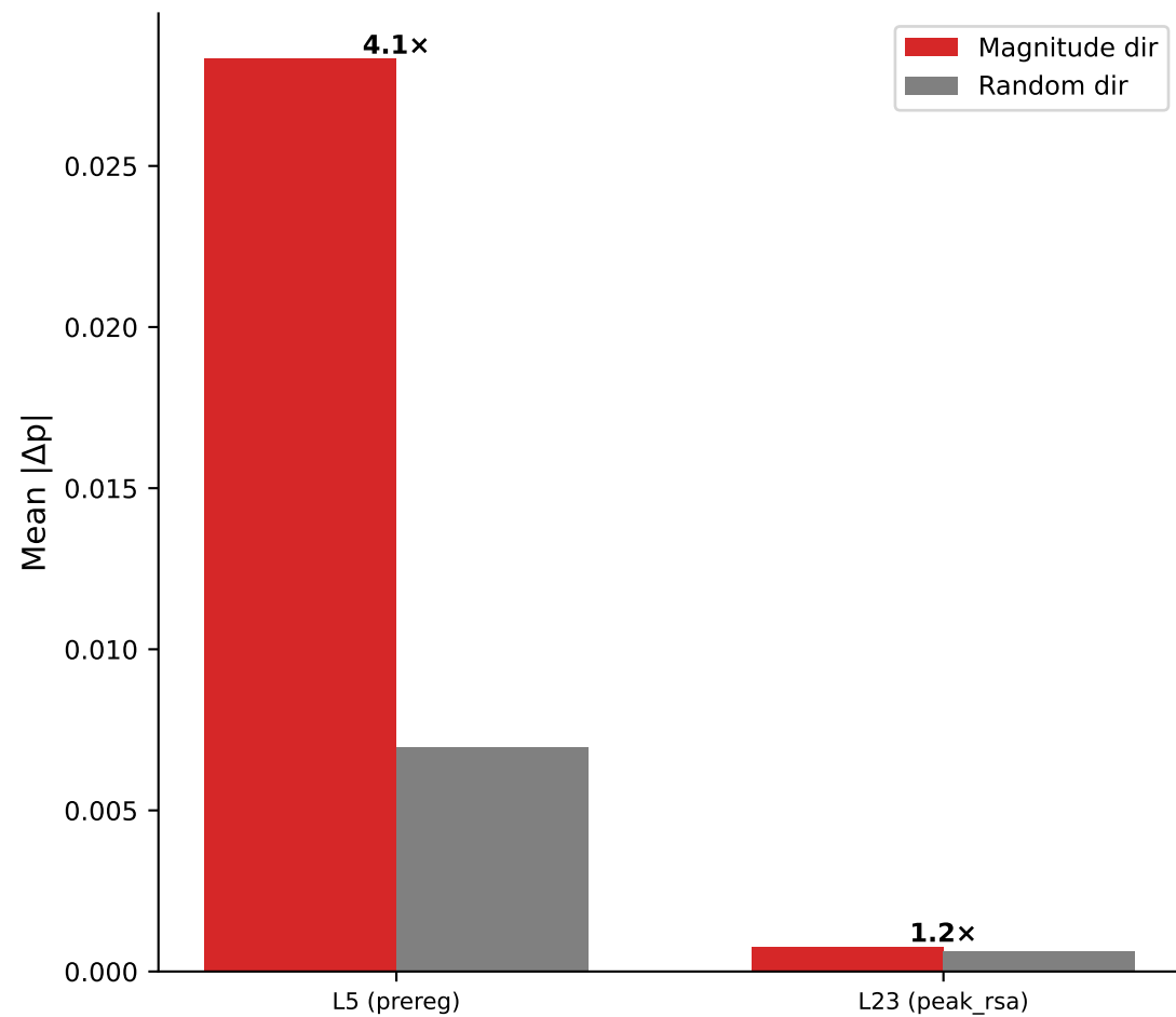
Llama-3-8B-Instruct
