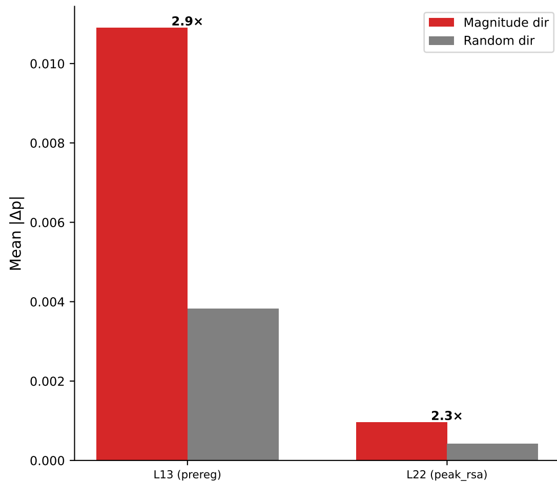
Mistral-7B-Instruct-v0.3
