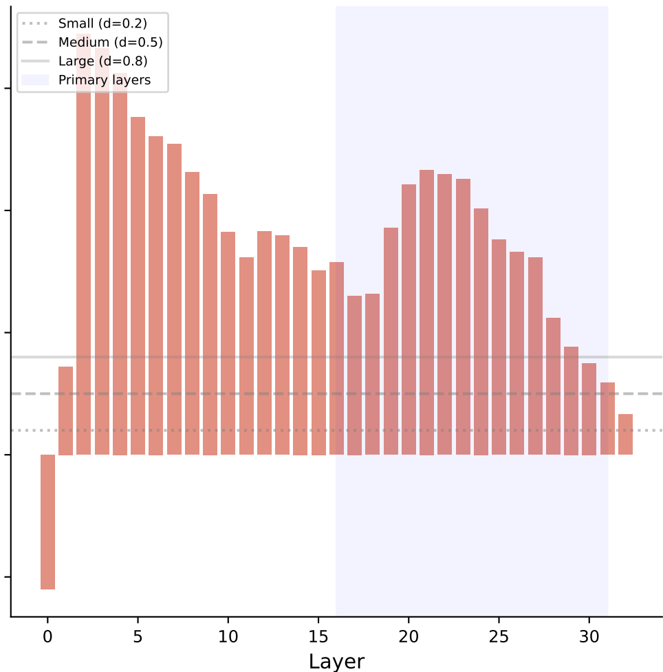
Mistral-7B-Instruct-v0.3
