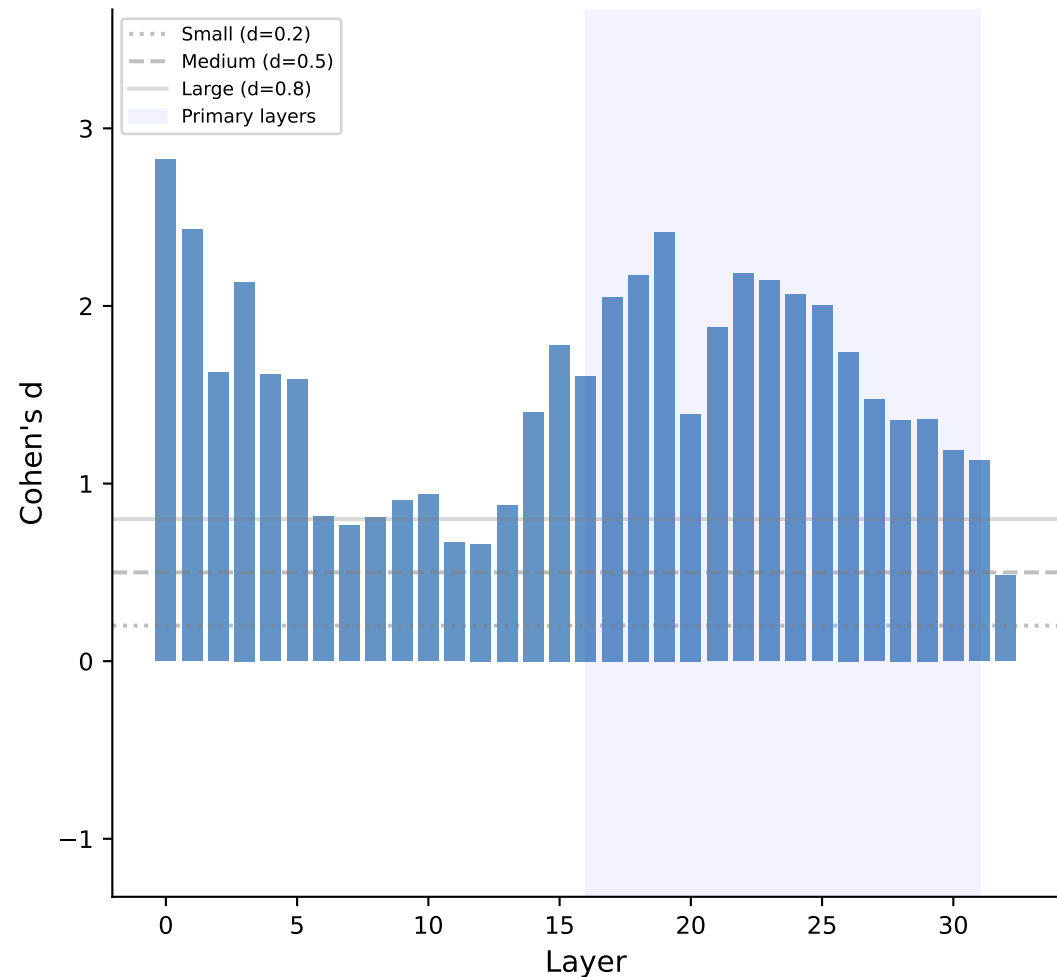
Llama-3-8B-Instruct
