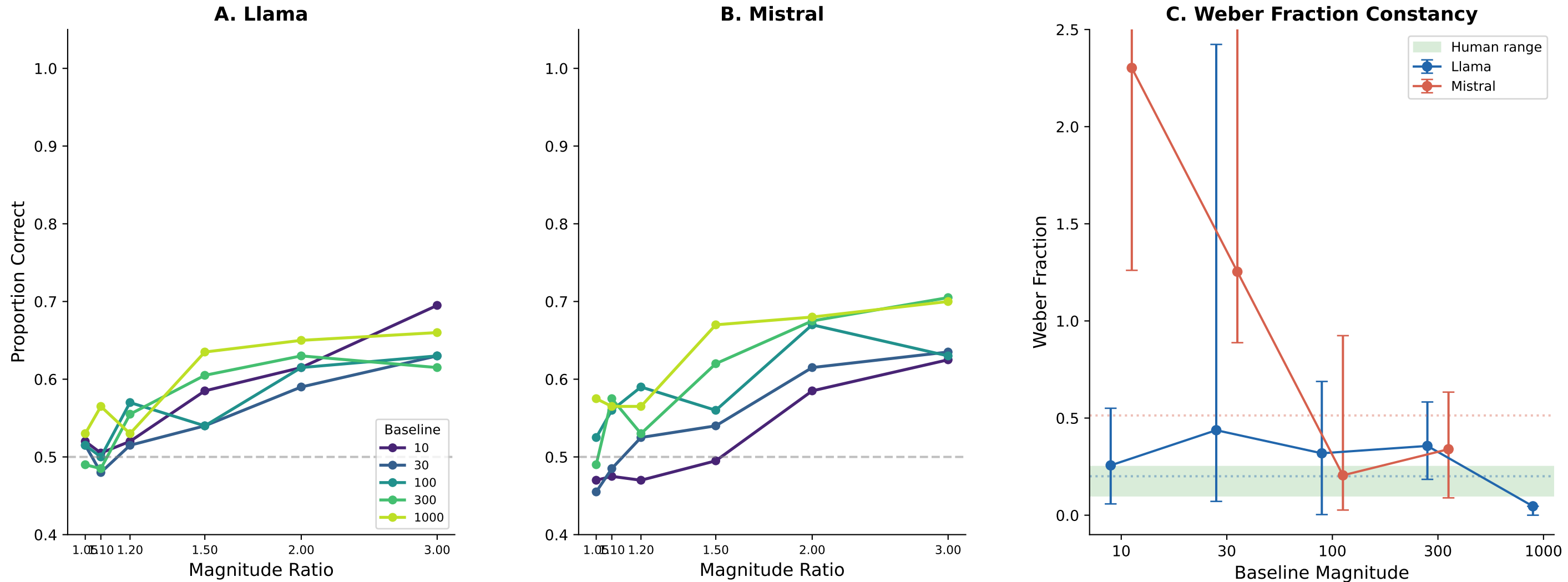
Figure 2. Behavioural Weber's Law: Llama shows ratio-dependent discrimination in the human range; Mistral does not.
