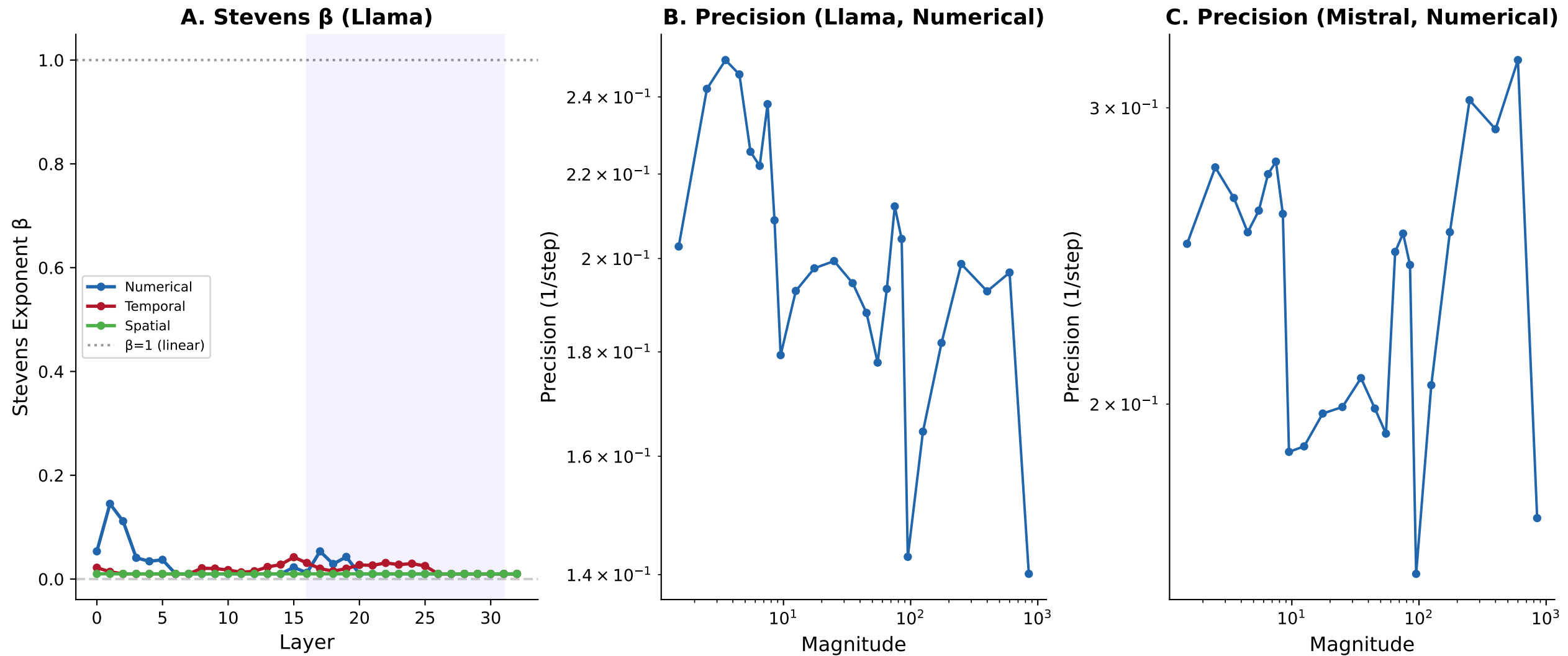
Figure 3. Compression is maximal ( \beta \approx 0 ) and precision declines with magnitude, consistent with efficient coding.
