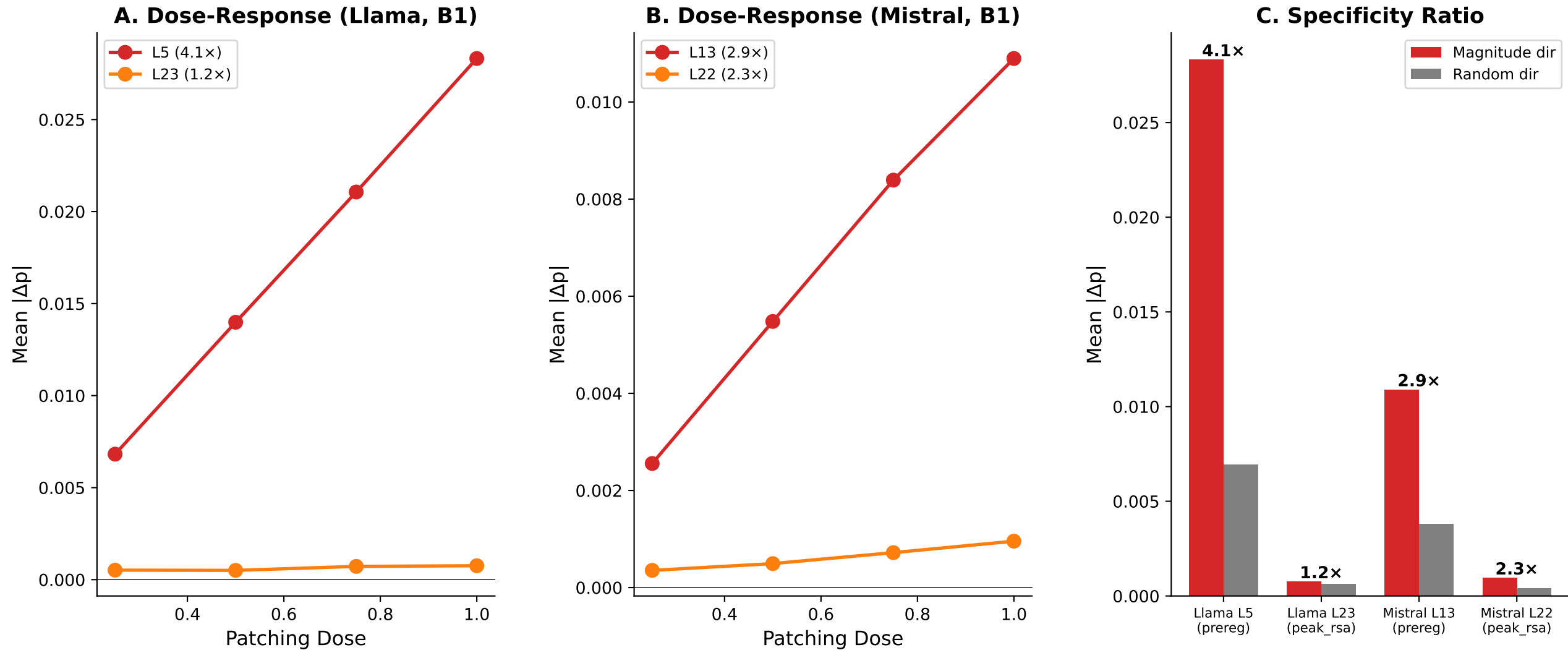
Figure 4. Magnitude subspace is causal at early layers for approximate tasks, but decorative where geometry is strongest.
