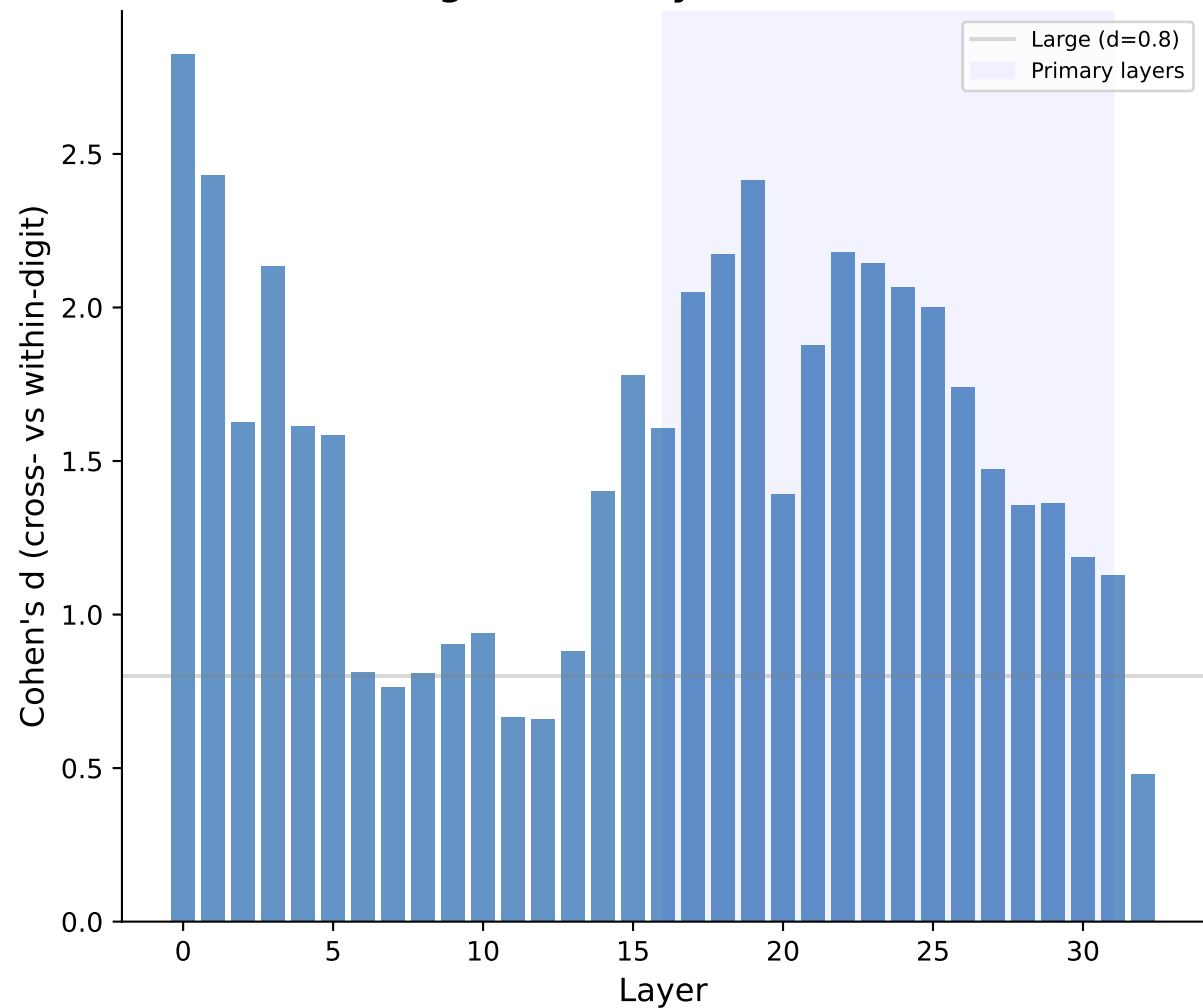
Figure 5. Digit-boundary effects are real but subordinate: log-magnitude dominates variance at all layers.
