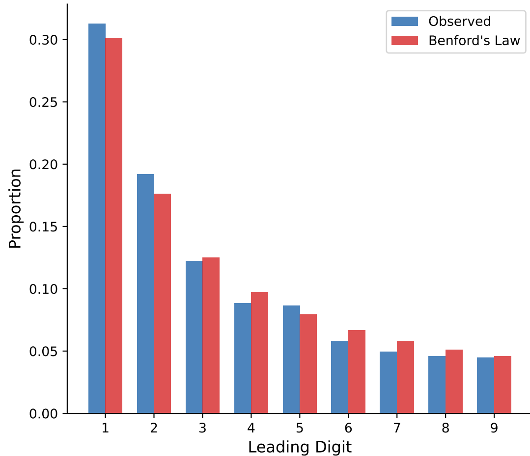
Figure 6. Natural language integer frequencies approximate a 1/s prior, grounding the efficient coding prediction.
