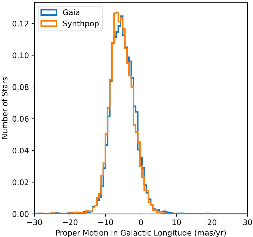
Comparison of Gaia vs. Synthpop Proper Motions ( l=0.0^\circ , b=5.0^\circ , G<20 )
