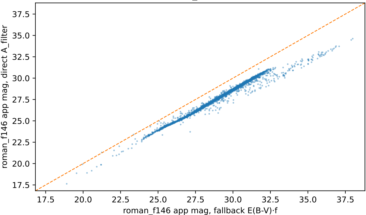
l=0.0, b=0.0: direct extinction vs fallback extinction
