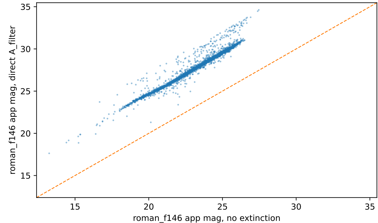
l=0.0, b=0.0: direct A_filter vs fallback E(B-V)·f
