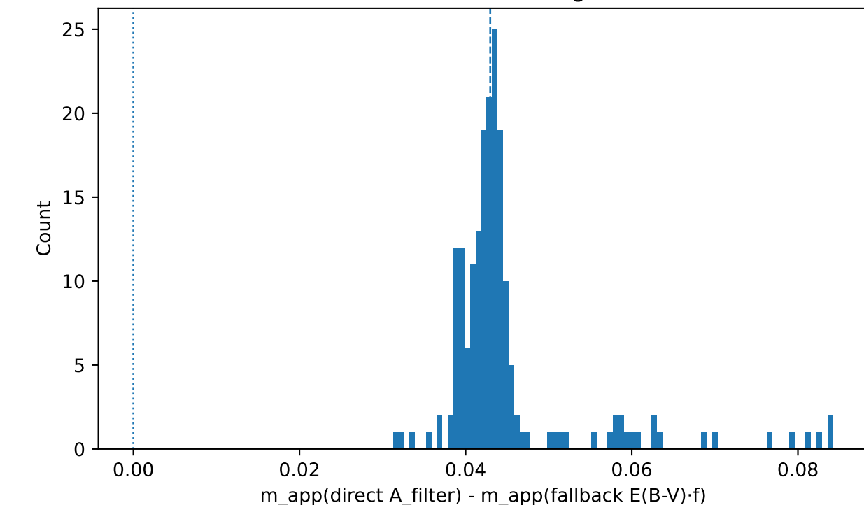
l=3.0, b=-3.0: measured vs expected delta
