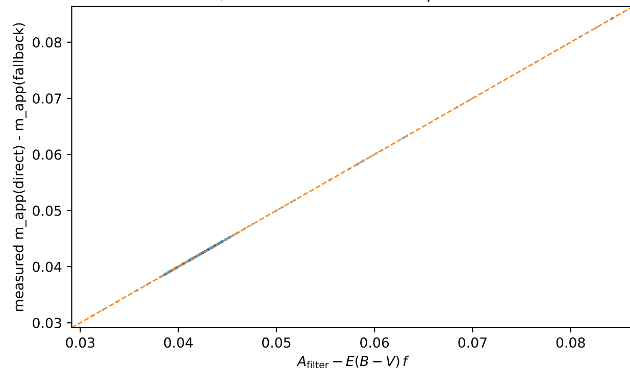
l=3.0, b=-3.0: residual from expected relation
