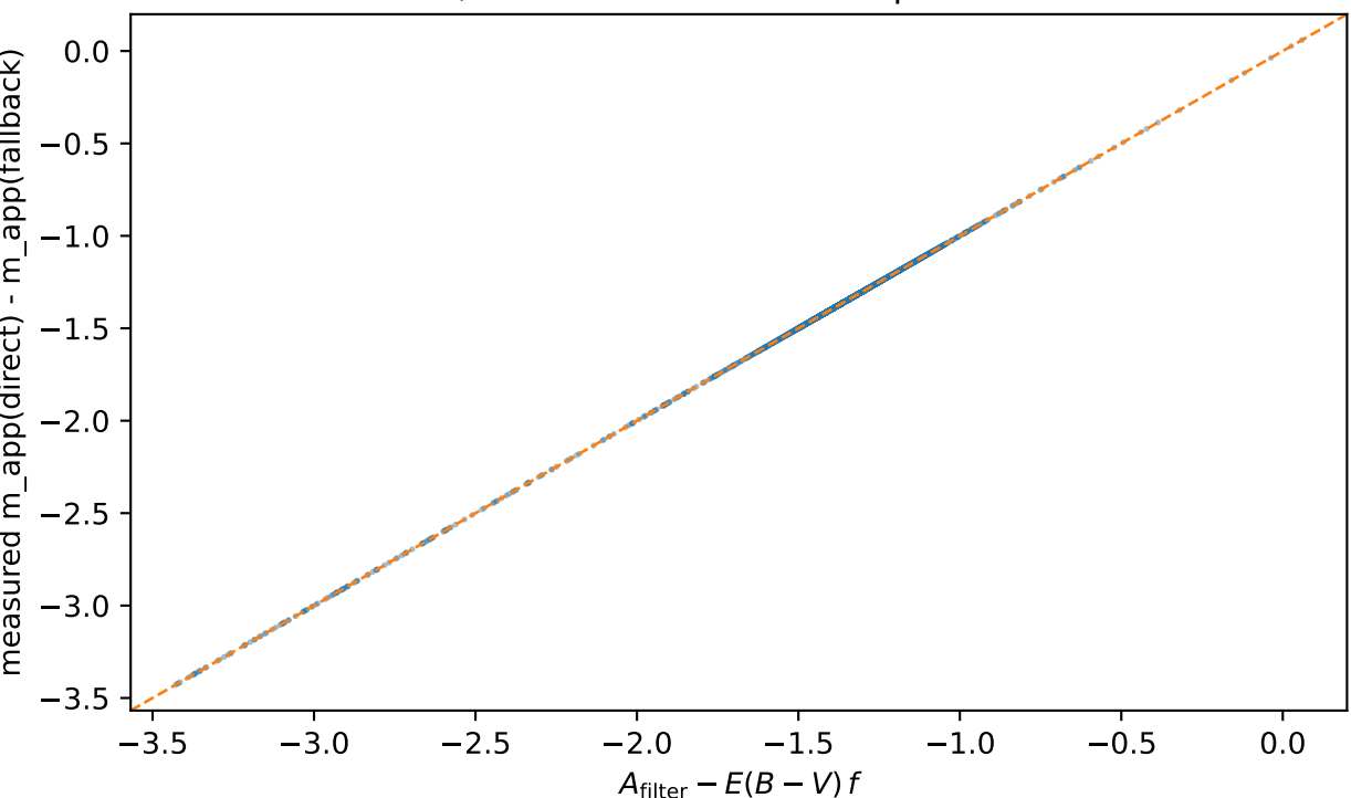
l=0.0, b=0.0: residual from expected relation
