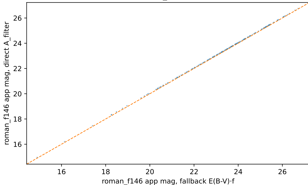
l=3.0, b=-3.0: direct extinction vs fallback extinction
