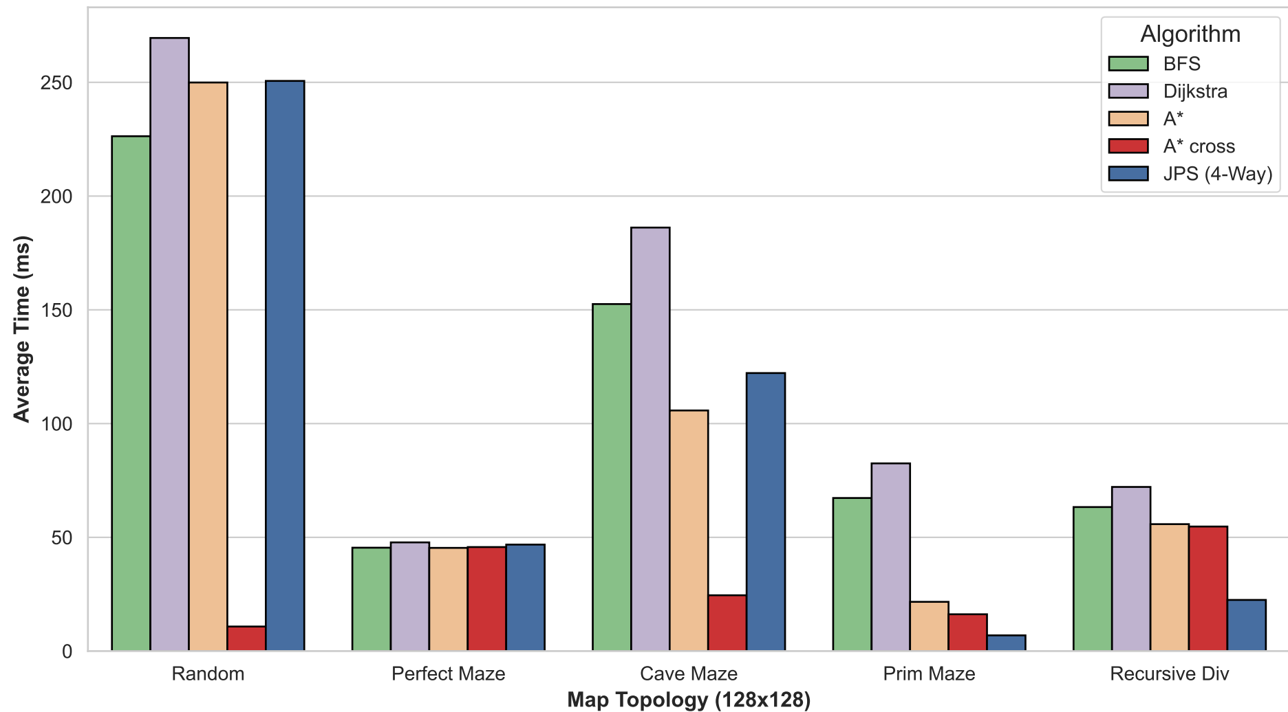
Algorithm Robustness Across Different Map Topologies
