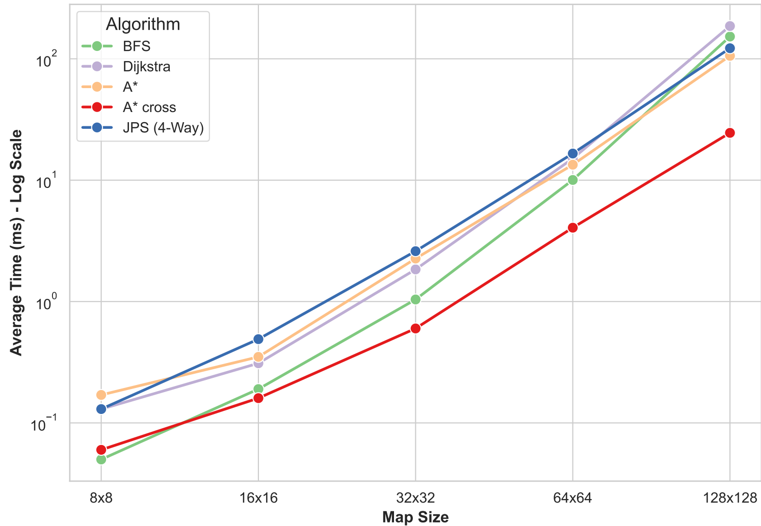
Scalability of Algorithms on Cave Maze
