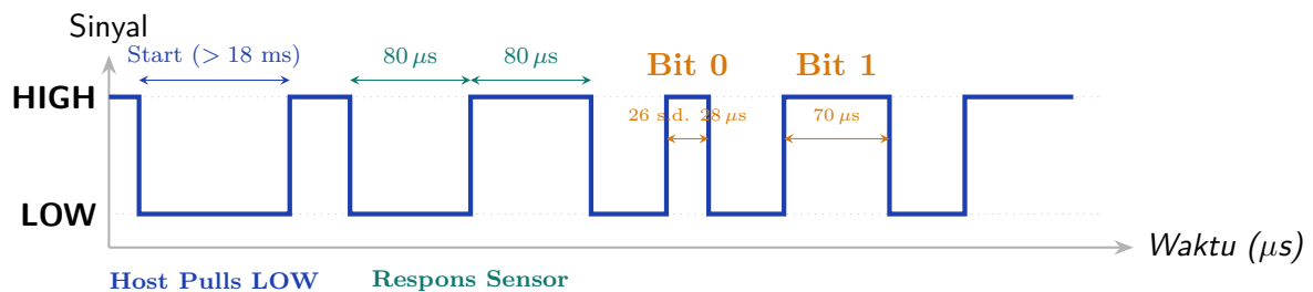
Gambar 11: Diagram pewaktu ( timing diagram ) protokol komunikasi single-bus DHT22.
