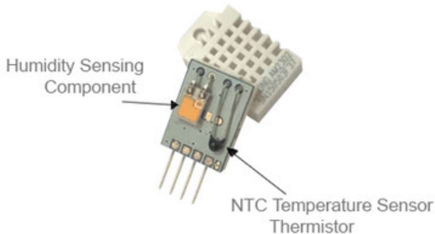
Gambar 10: Elemen sensoris AM2302/DHT22.
