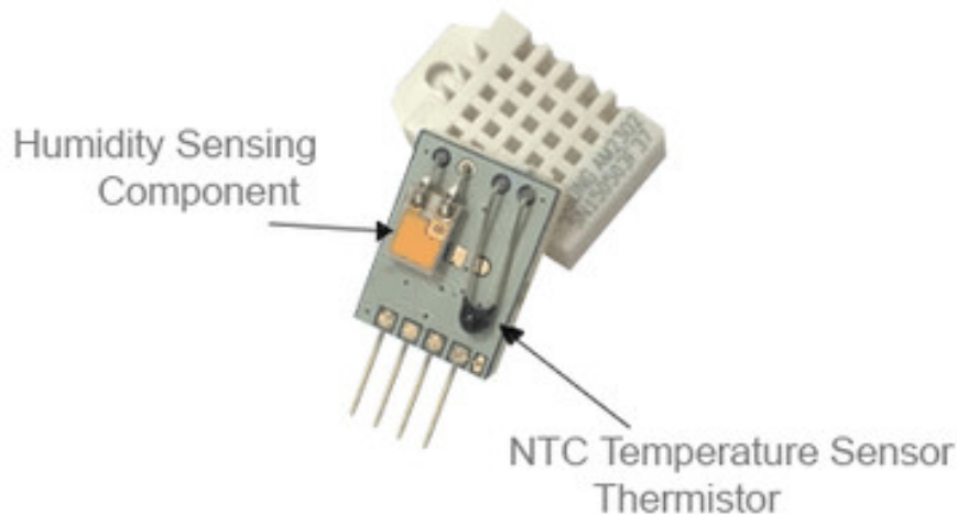
Gambar 10: Elemen sensoris AM2302/DHT22.
