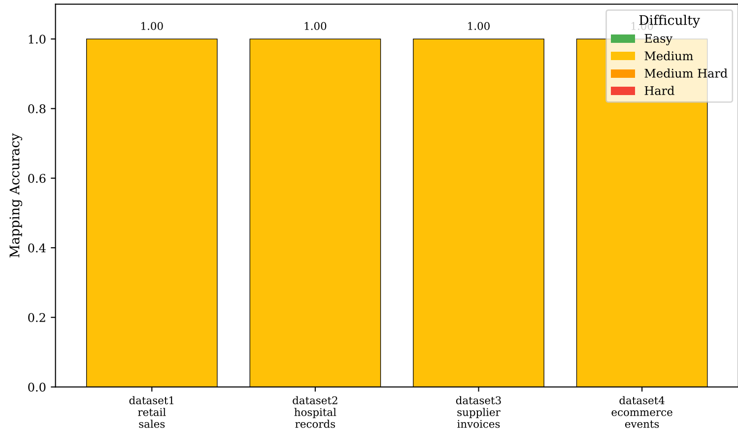
Schema Mapping Accuracy by Dataset
