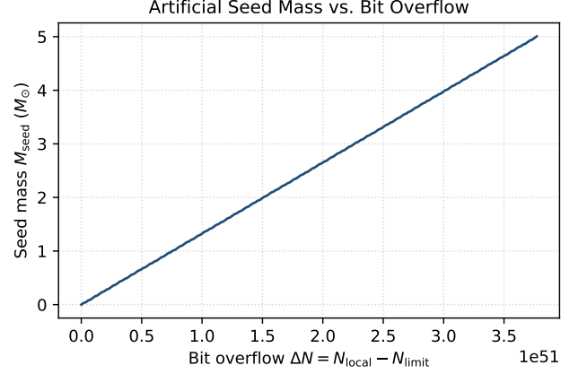
Fig. 2. Artificial ghost-seed mass as a function of bit overflow \Delta N = N_{local} - N_{limit} .
