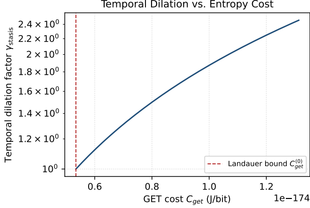
Fig. 1. Newton-lock temporal dilation factor \gamma_{stasis} versus GET cost C_{get} . The dashed vertical line marks the cosmic Landauer bound C_{get}^{(0)} .
