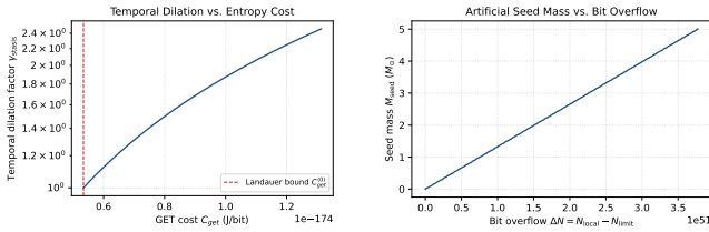
Fig. 1. Newton-lock temporal dilation factor \gamma_{\text{stasis}} versus GET cost C_{\text{get}} . The dashed vertical line marks the cosmic Landauer bound C_{\text{get}}^{(0)} .
