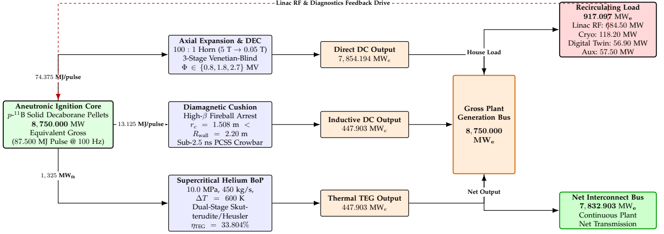
Fig. 1. Complete energy-flow topology of the SHBT-Graser plant: core yield partitioning into the DEC, inductive cushion, and thermal-TEG channels; gross-bus aggregation; and the 917.097 MW recirculating house load feeding back to the driver.
