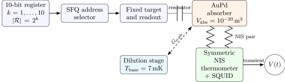
Figure 2: Inline apparatus schematic for the address-scaling test. The SFQ selector varies the active address depth while the same target and readout path deposit energy in the AuPd absorber; symmetric NIS junctions and a SQUID read the electron-temperature transient at the 7 mK stage.
