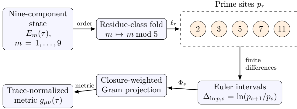
Figure 1: Prime-lattice RG folding. The ordered nine-component entropy state is folded by residue class onto the five prime sites; finite differences over the four logarithmic Euler intervals feed the closure-weighted Gram projection.
