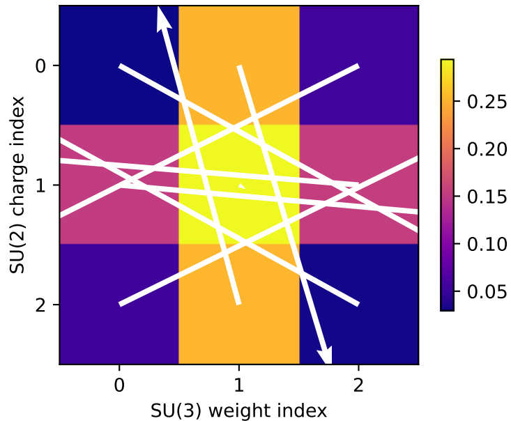
Excited Shannon contributions
