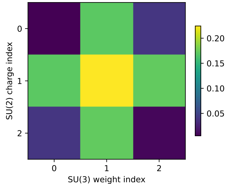
Baseline Shannon density
