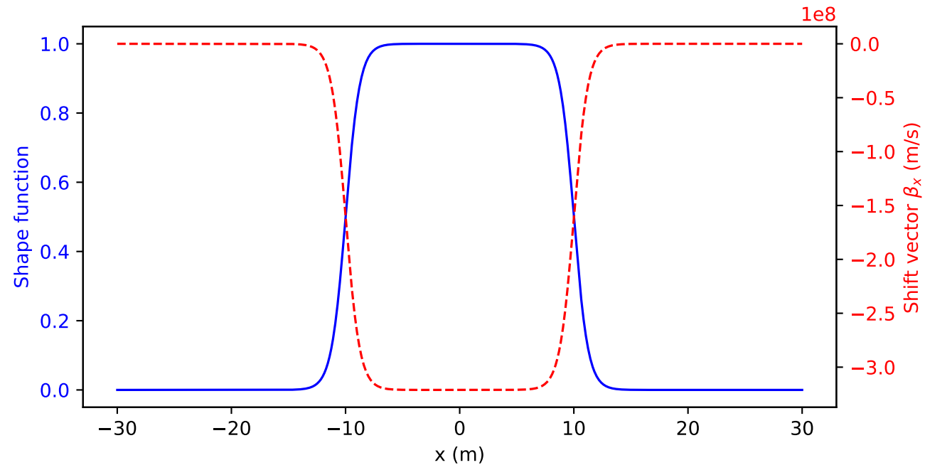
Warp bubble profile
