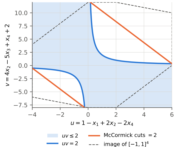
(a) uv \leq 2 and its McCormick cuts
