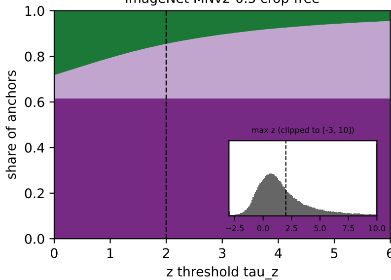
ImageNet MNv2-0.5 crop-free
