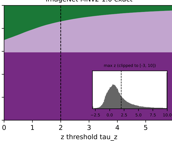
ImageNet MNv2-1.0 exact
