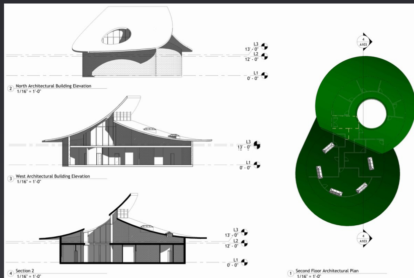
ELEVATIONS &amp; SECTIONS
