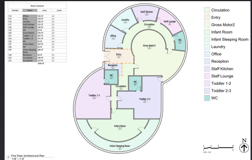
FLOOR PLAN
