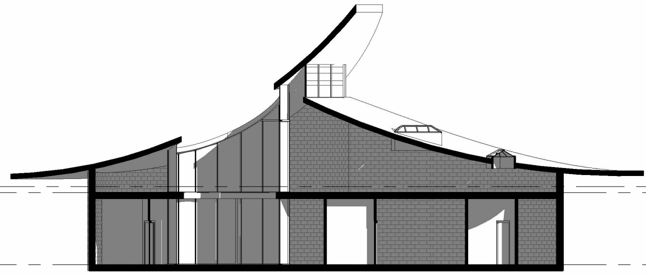
④ Section 2 1/16" = 1'-0"
