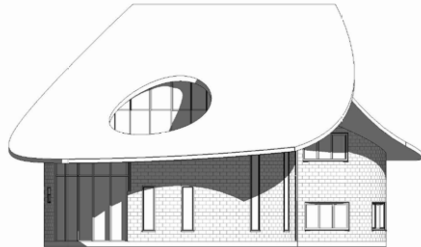
① North Architectural Building Elevation 1/16" = 1'-0"
