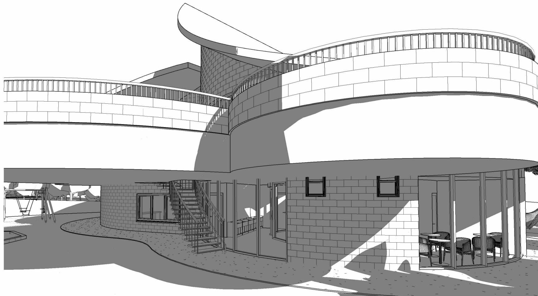
3 Exterior View Stairs
