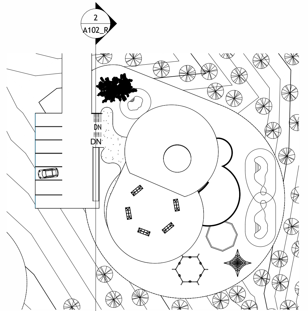
1 Site Plan 1" = 40'-0"
