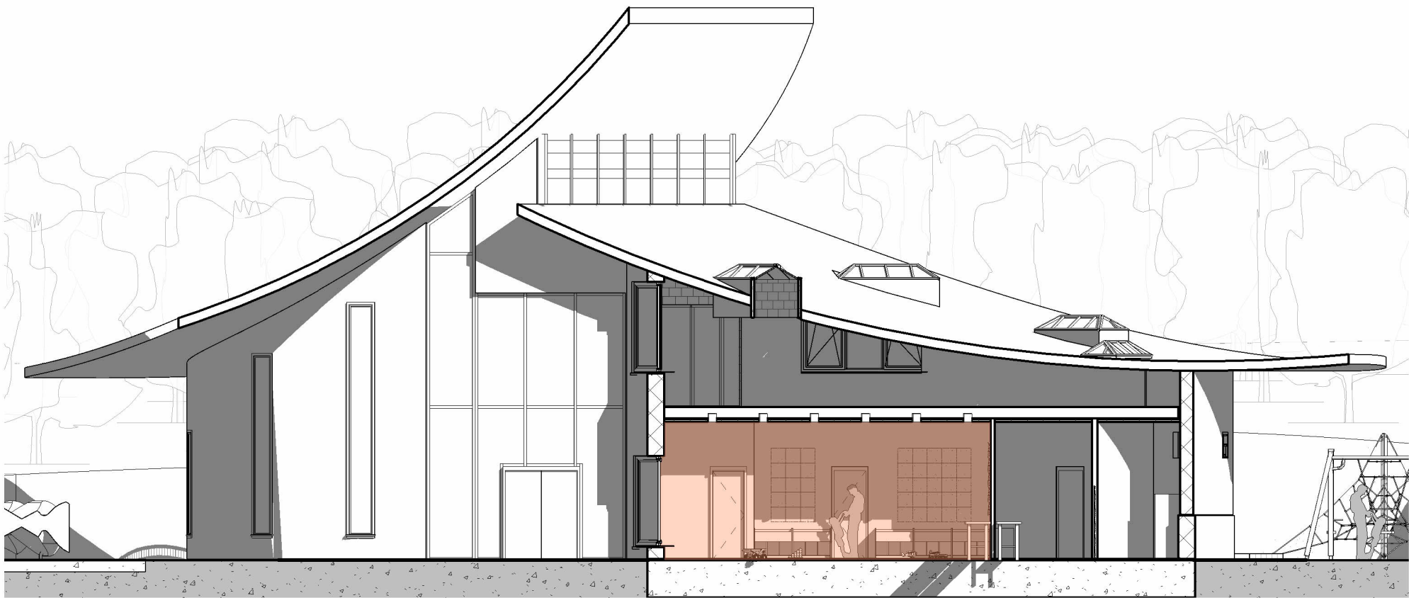
③ Section 5 3/32" = 1'-0"
