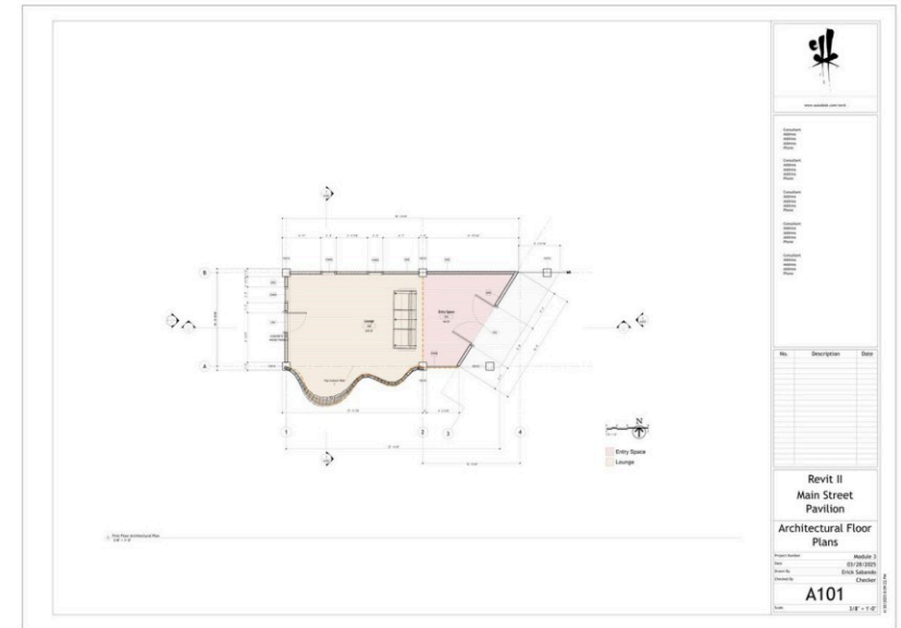
FLOOR PLAN - A101
