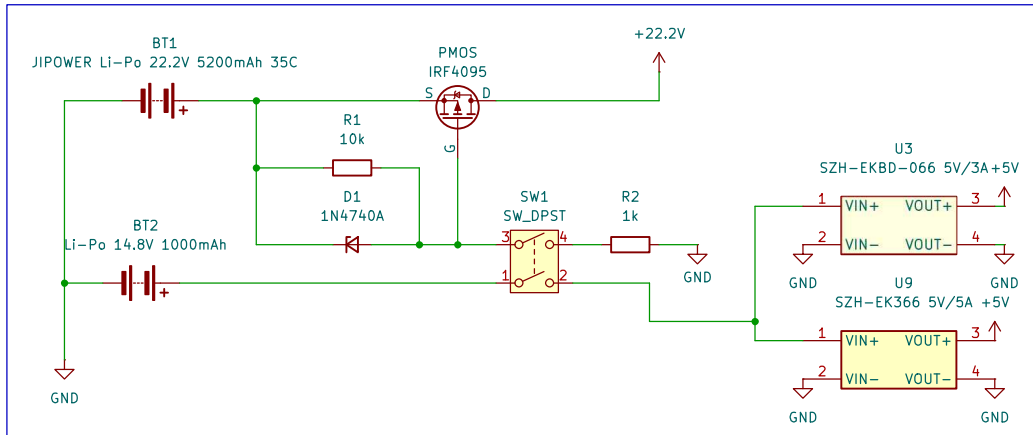
Power_Distribution
