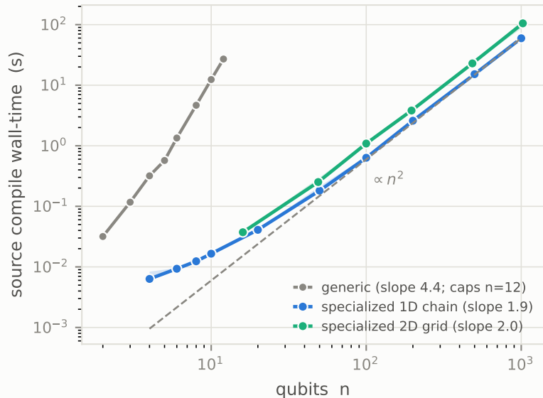
(a) Source compilation \rightarrow schedule ops + ledger
