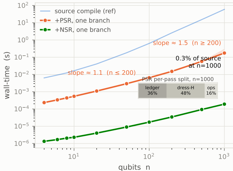
(b) Incremental cost per derivative branch
