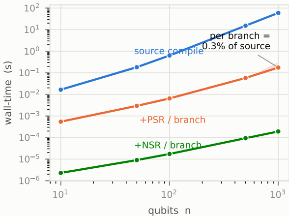
Derivative compile cost over the source path
