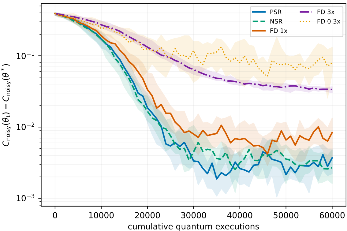
F-loop (REAL estimators) — TFIM P=4 descent, emulated noisy cost ( T/T_2^*=0.15 , B=1000/\text{grad} )
