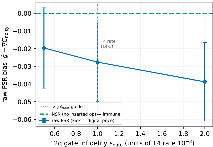
C3 — PSR kick-gate bias vs NSR immunity ( T/T_2^*=0.15 , coh-frac 0.5)
